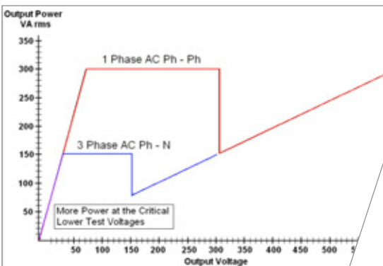
PowerV™ technology guarantees a flat curve from 30 to 150 V, eliminating range switching
