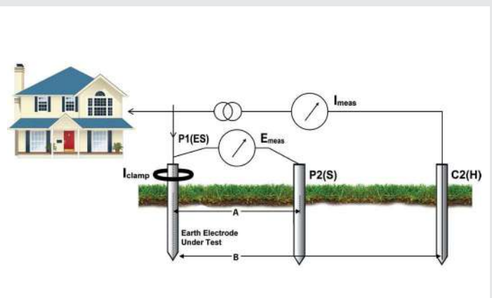
The current I_{clamp} is the portion of I_{meas} which flows into the electrode-under-test. I_{meas} - I_{clamp} flows into the rest of the connected Earthing system. Electrode resistance, R = E_{meas} / I_{clamp}
