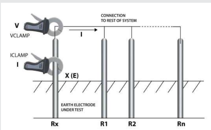
Schematic for two-clamp stakeless resistance measurement
